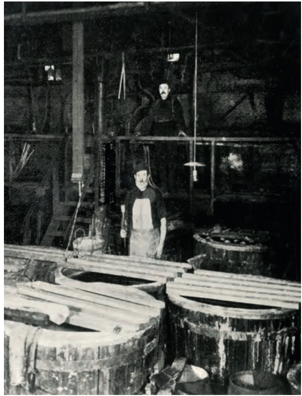
Wet chemical workshops at the vitriol smelter at Elbstrasse. This was the location where copper vitriol was produced. The foreground of the photo shows crystallization tanks hung with lead bars. Evaporating pans are standing on the platform in the background.
